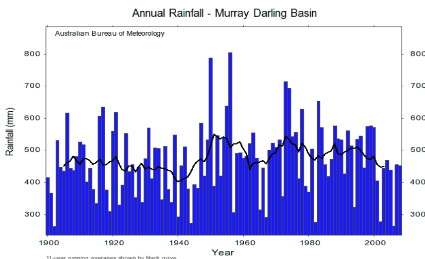
Fig. 2. Murray-Darling rainfall record, 1900-2008. ( http://www.bom.gov.au/cgi-bin/climate/change/timeseries.cgi?graph=rain&area=mdb&season=0112&ave_yr=11 ).
